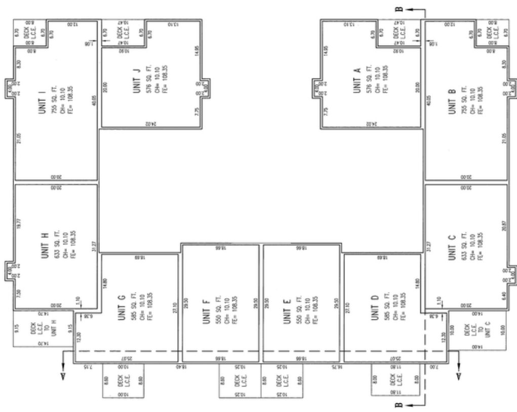
SECOND STORY INTERIOR WALLS 0.00' WEL, OR AS NOTED EXTERIOR WALLS 0.00' WEL, OR AS NOTED
